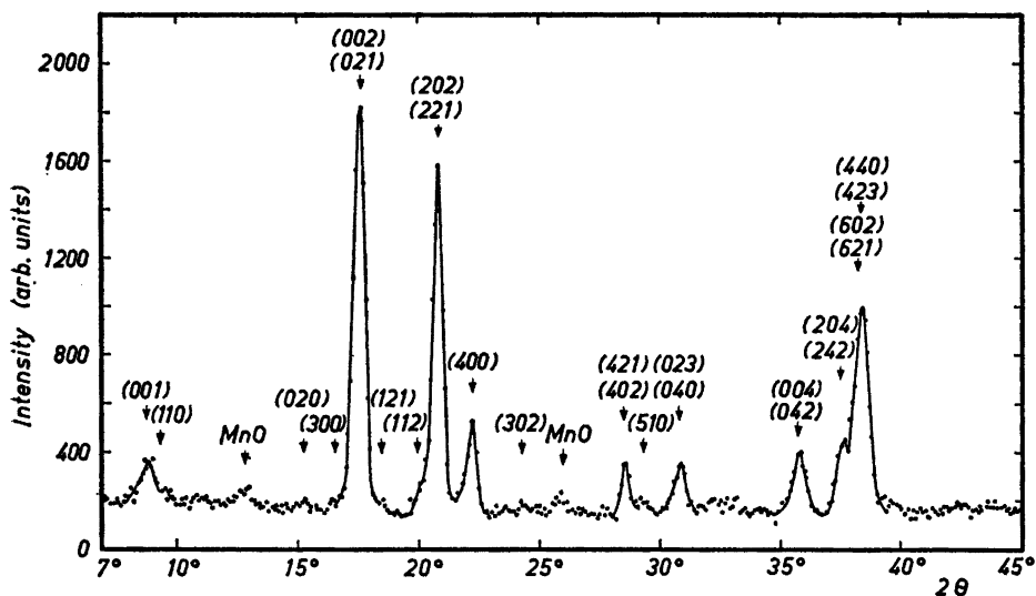
Fig. 6. Neutron diffraction diagram of quenched phase at 5^\circ\text{K} , \lambda = 1.147 \text{ \AA} .
