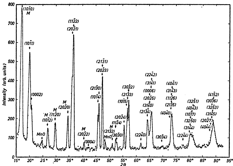
Fig. 1. Neutron diffraction diagram at 20°C of the annealed phase, \lambda = 1.101 Å. Reflections with a significant magnetic contribution are marked with an M.
